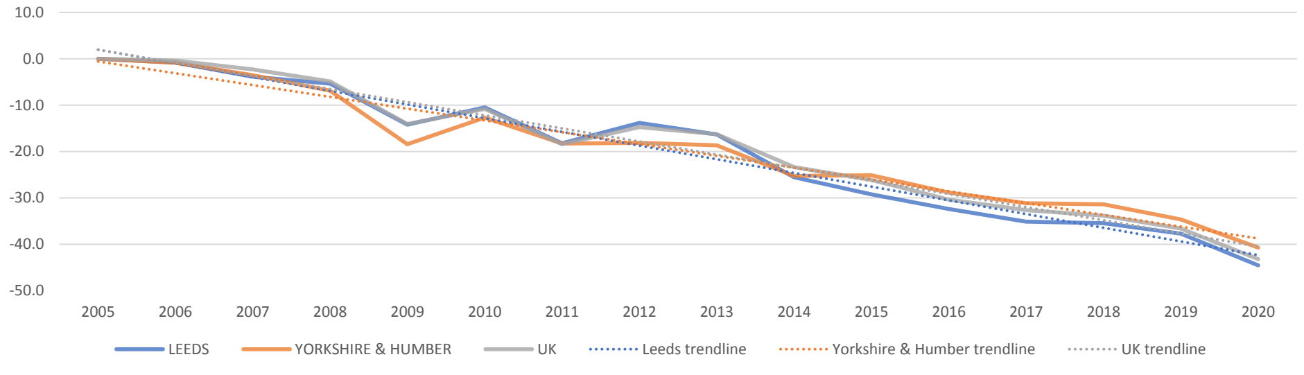
CHART 15: REDUCTION IN CARBON EMISSIONS (%) BY GEOGRAPHICAL AREAS; 2005-2020
