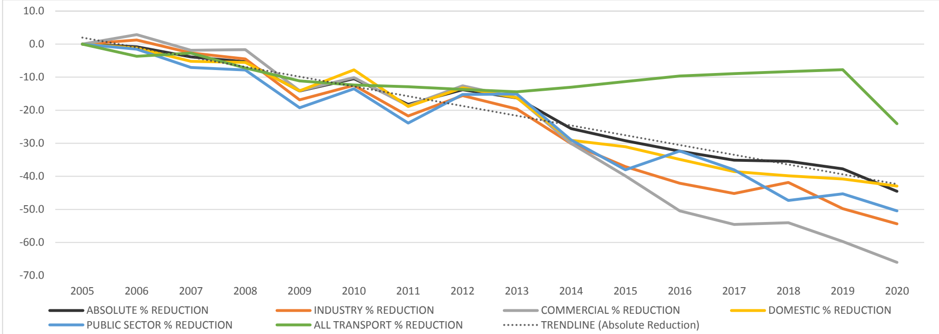
CHART 16: REDUCTION IN CARBON EMISSIONS (%) IN LEEDS BY MAJOR EMITTER; 2005-2020
