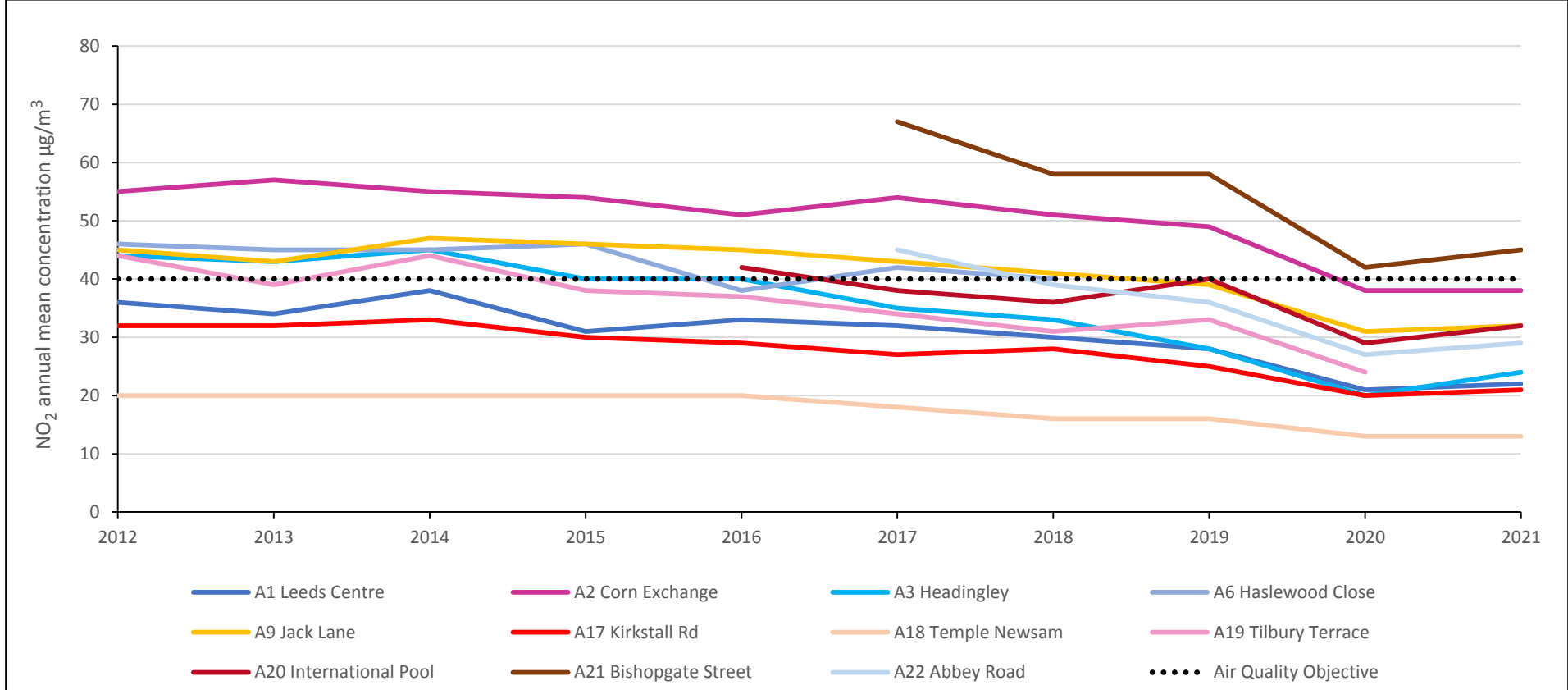
CHART 22: LEEDS NO2 AUTOMATIC AIR QUALITY MONITORING SITES; 2012-2021
